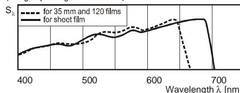
Relative spectral sensitivity (wedge spectrogram at 2850 K)
